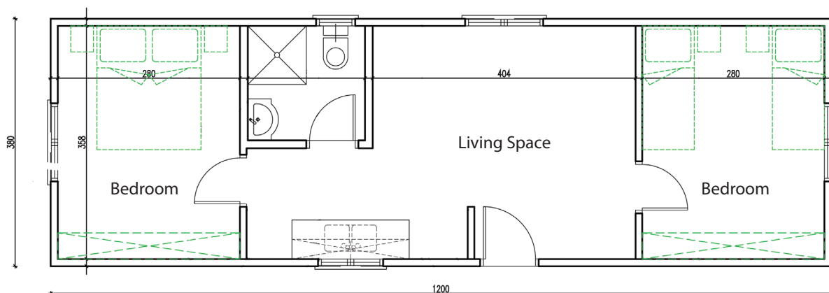
The modular home floor plan
